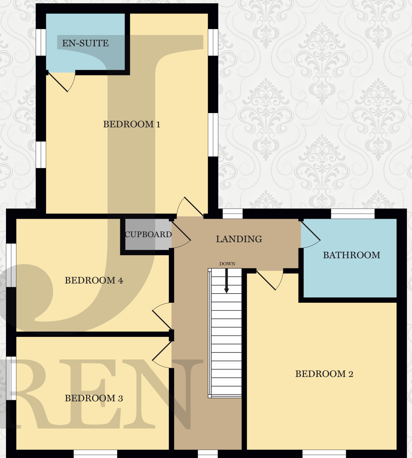
1 ST FLOOR
