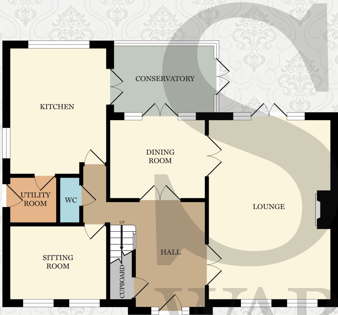
GROUND FLOOR
